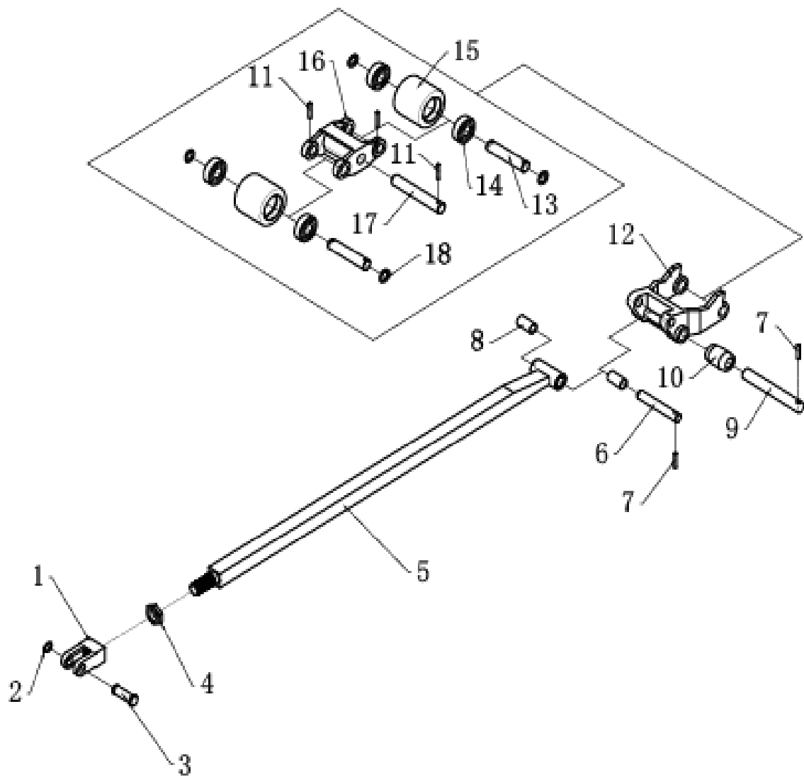
Fig.3 Push rod front wheel assembly
