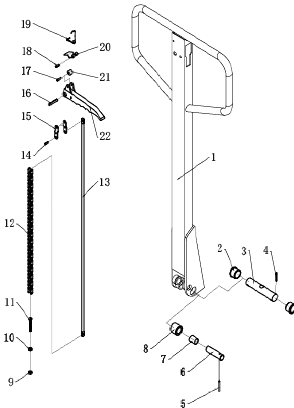
Fig.4 Handle assembly
