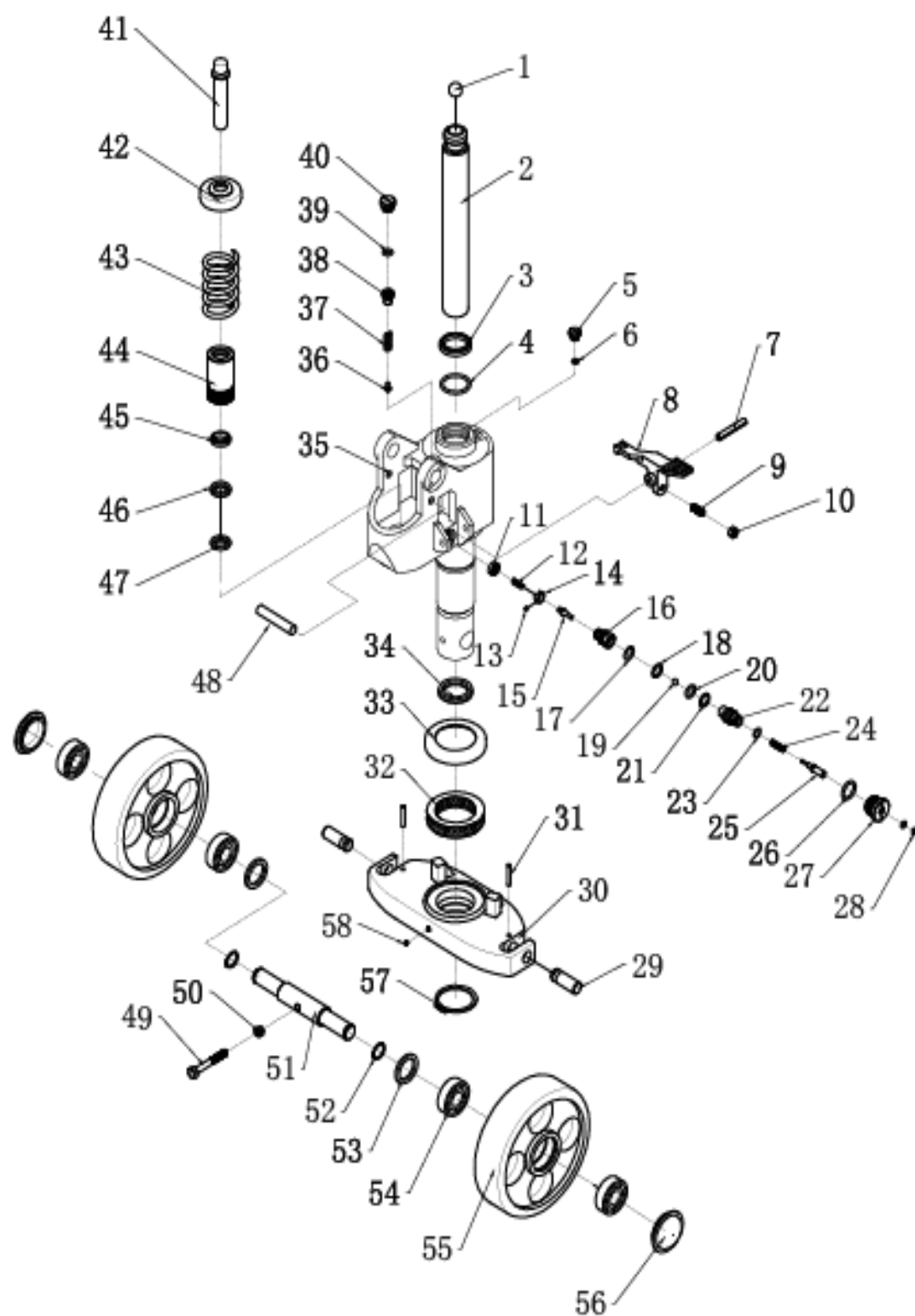
Fig.2 Cylinder pedestal assembly
