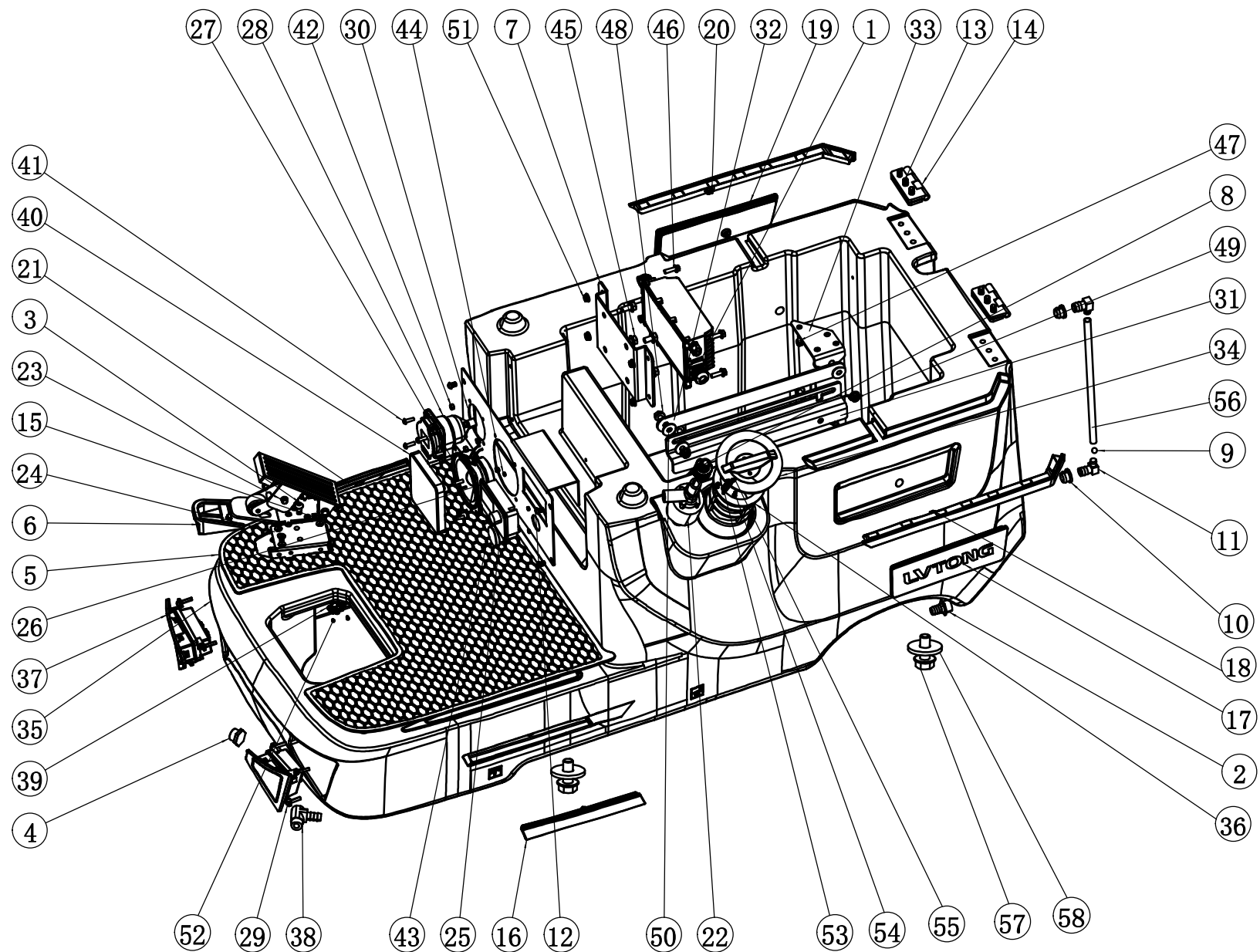
清水箱组件零件图 Clean Water Tank Assembly Parts List
