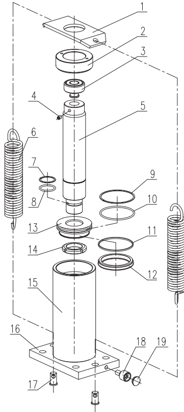
RAM PARTS LIST (figure b)
