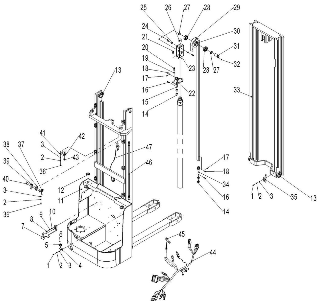
Fig.17 Mast assembly (Two-stage mast)
