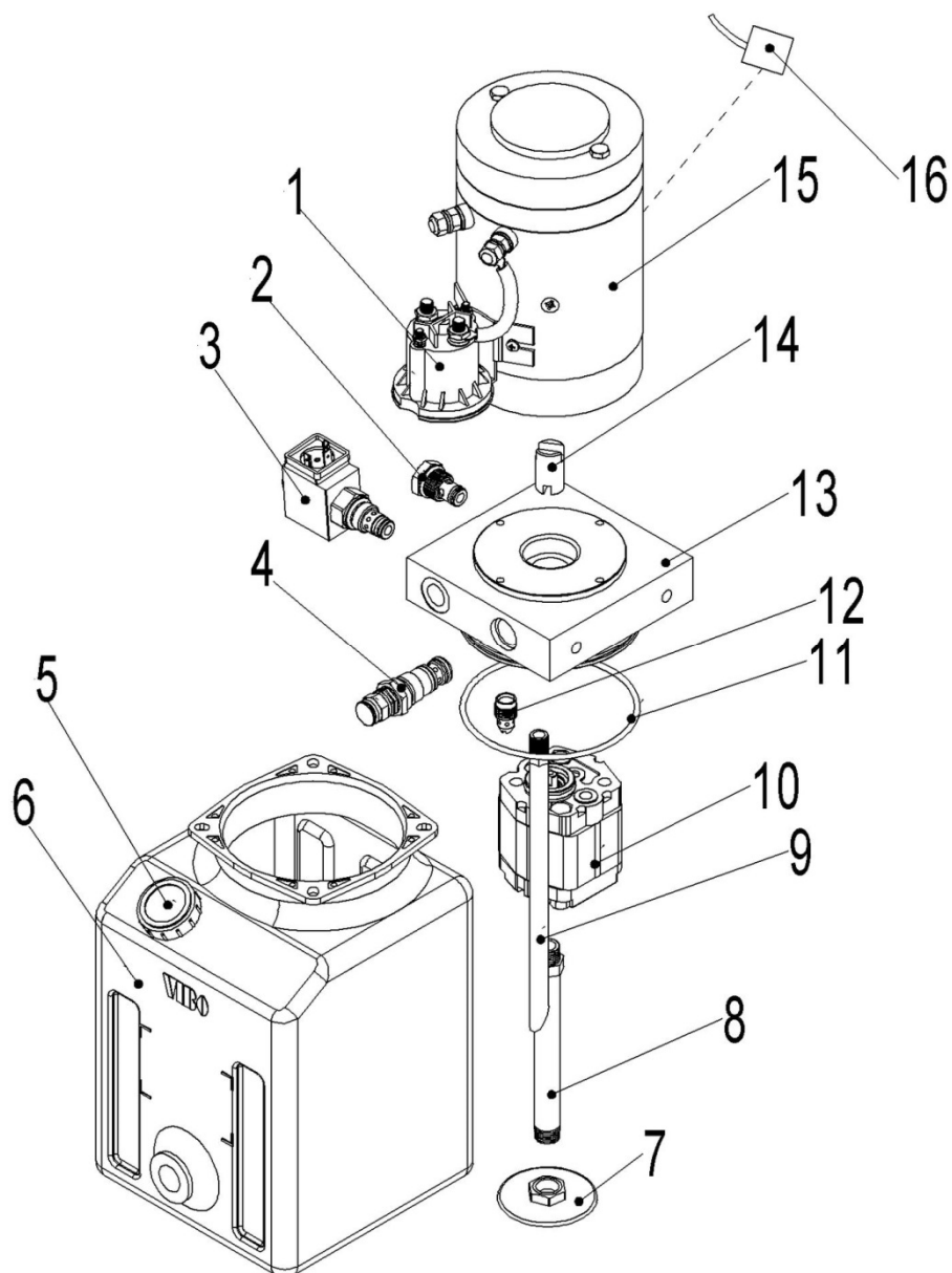
Fig.10 Hydraulic power unit
