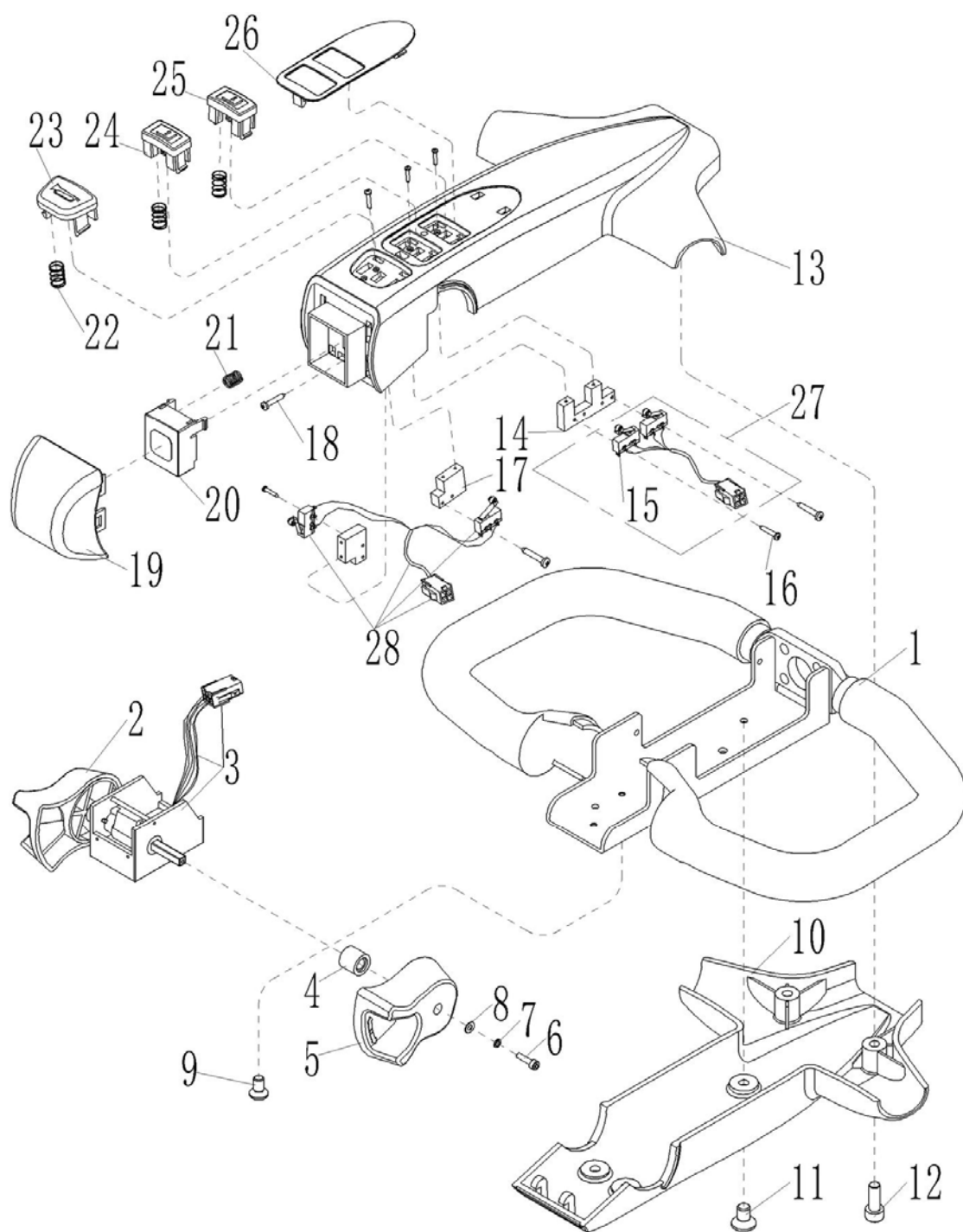
Fig.14 Tiller head components
