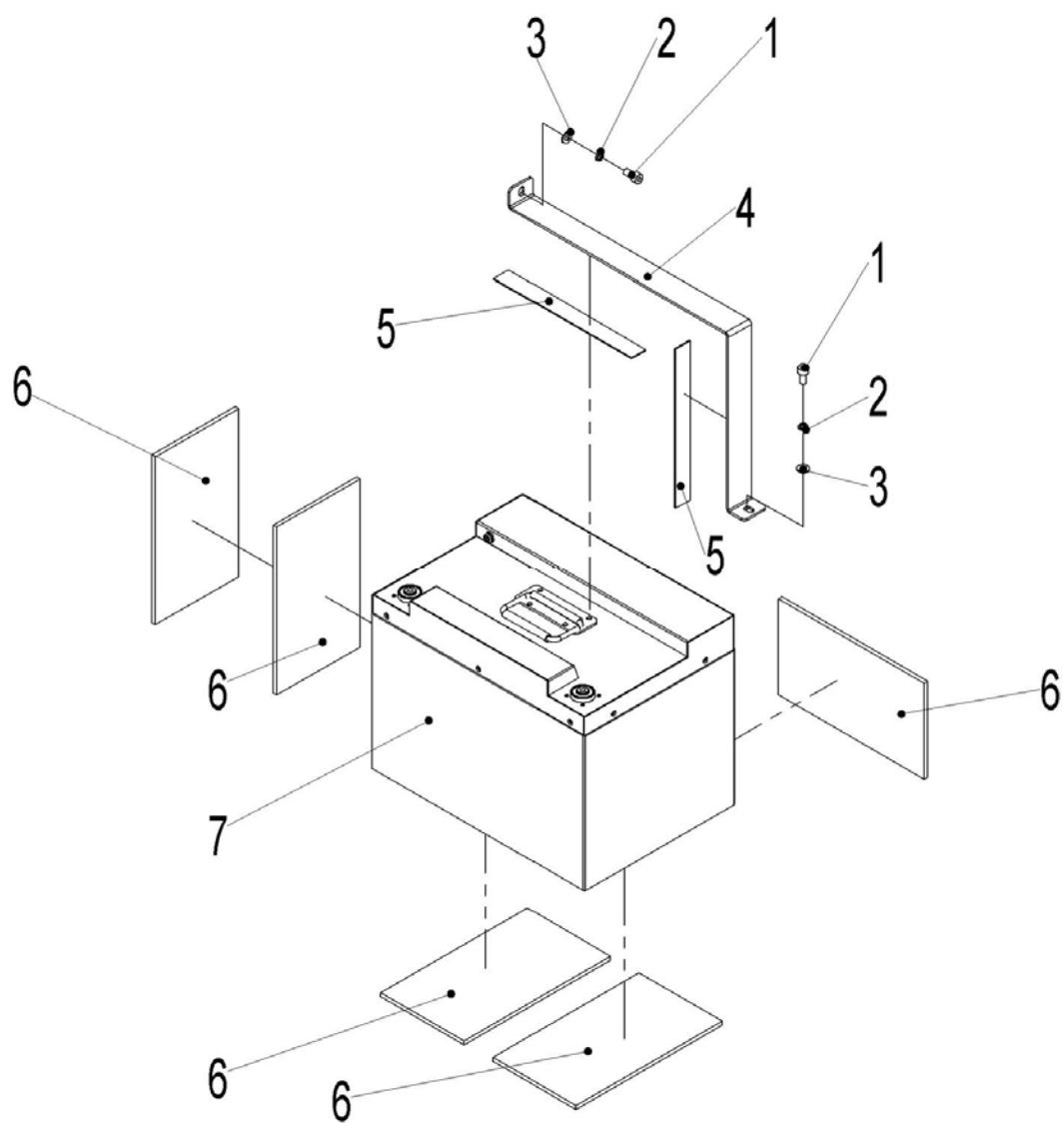
Fig.16 Battery components(ECL15N)
