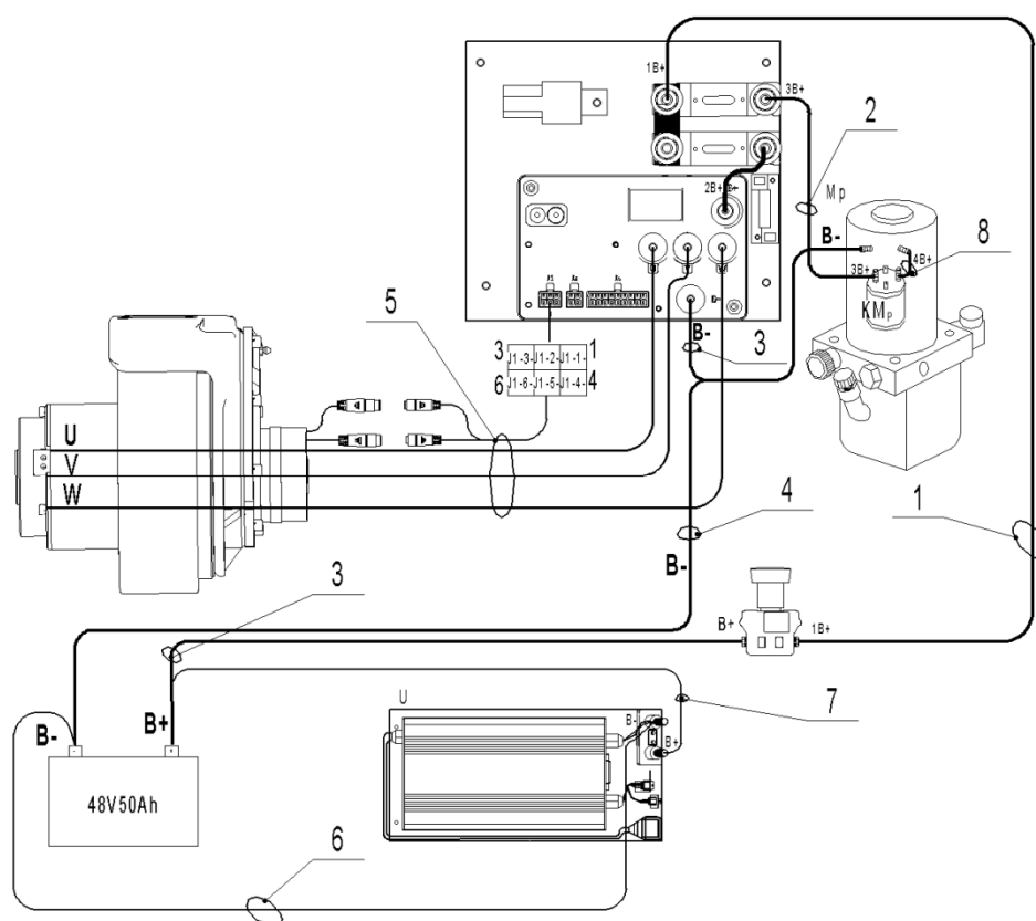
Fig.23 wiring harness(ECL15N)
