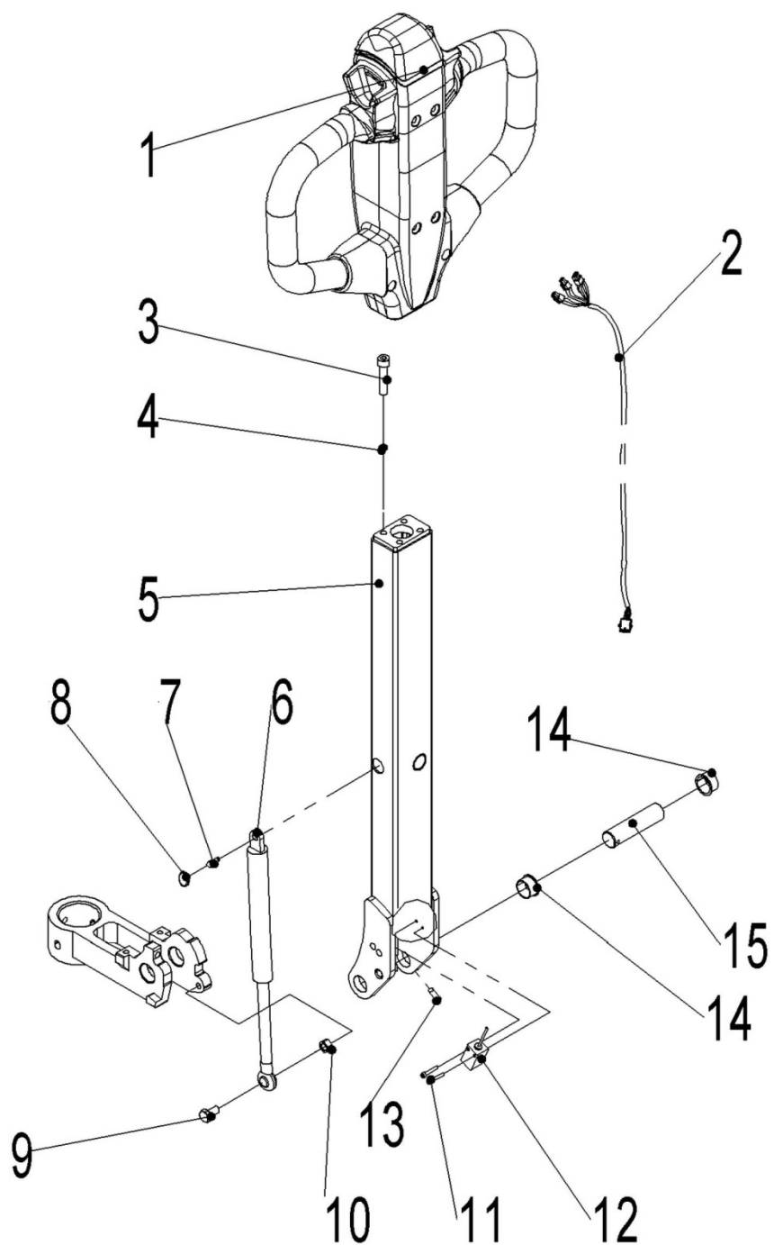
Fig.13 Tiller components
