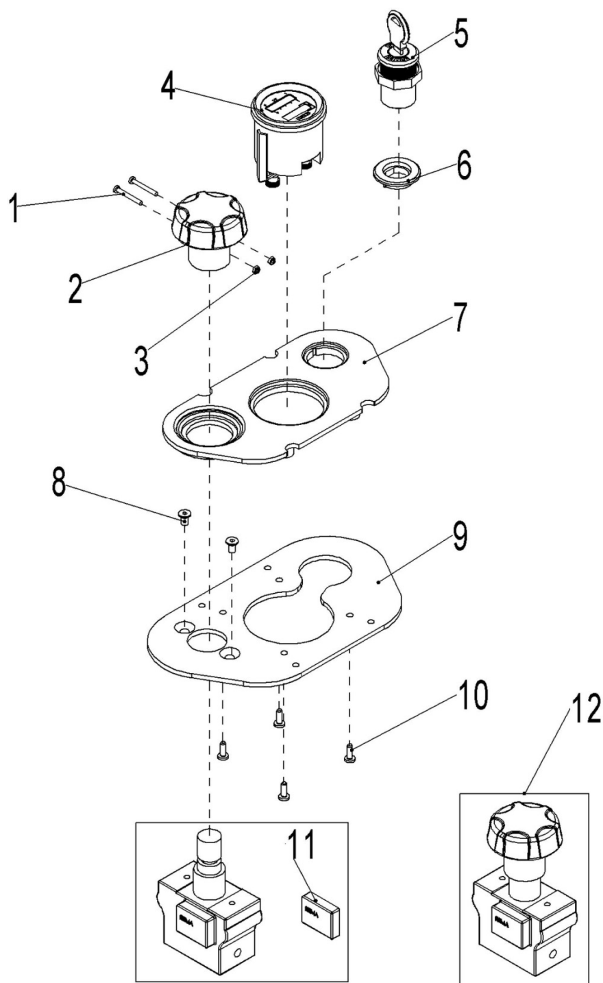
Fig.12 Panel components
