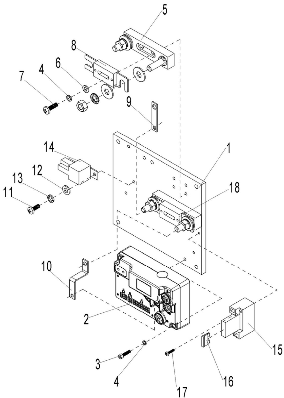
Fig.19 Controller components
