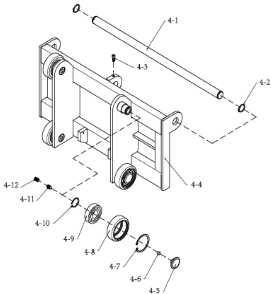
Fig.4 Lifting frame assembly
