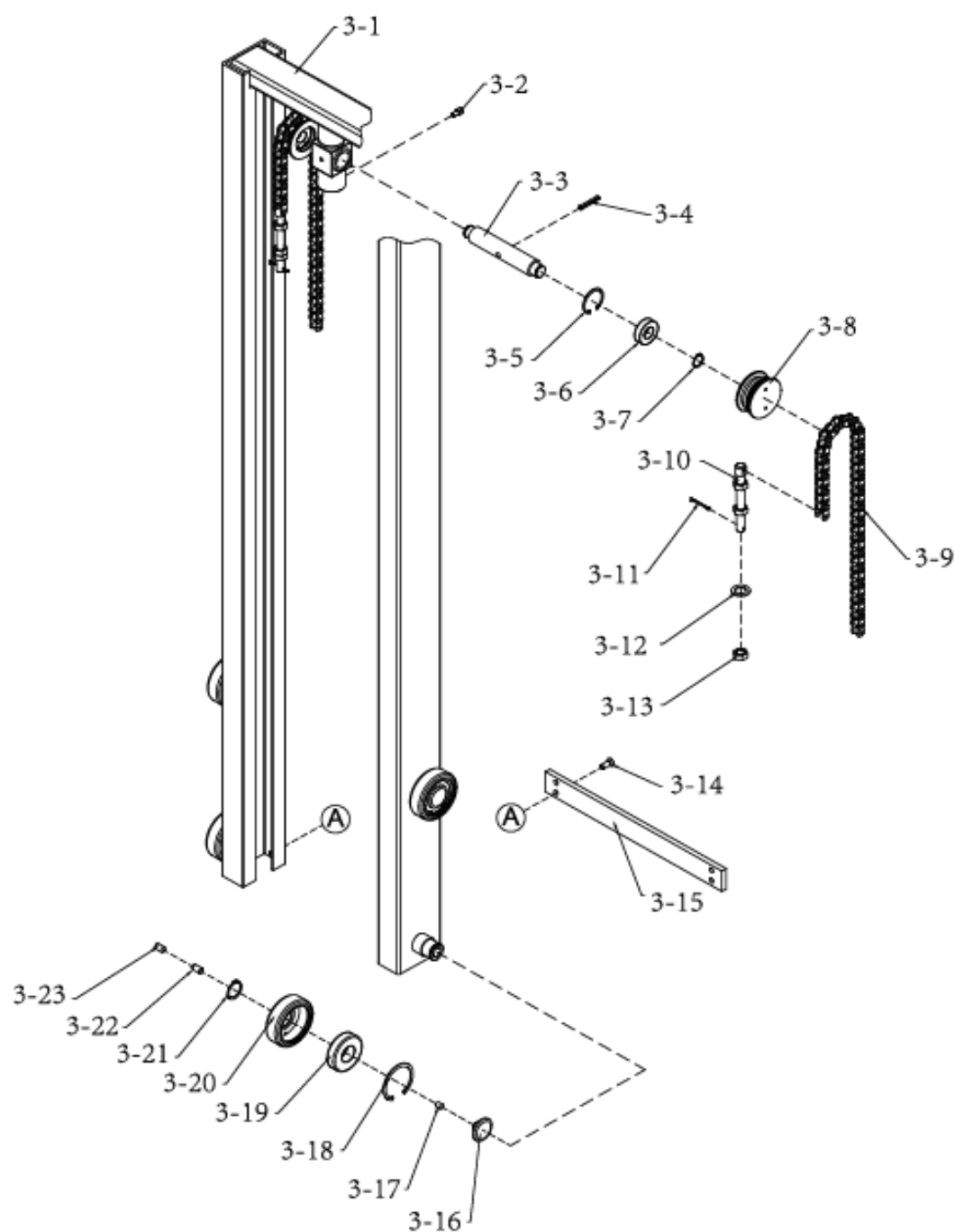
Fig.3 Inner door frame assembly
