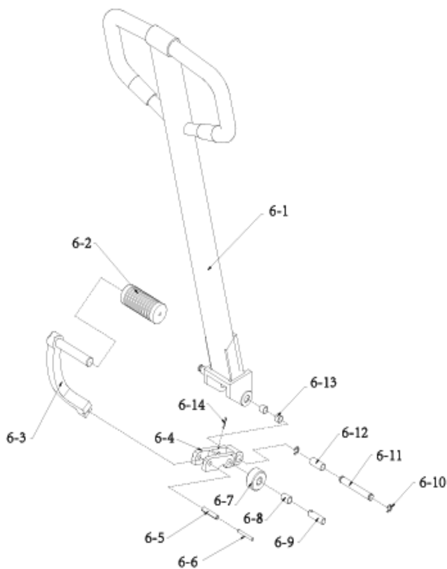
Fig.6 Control handle assembly
