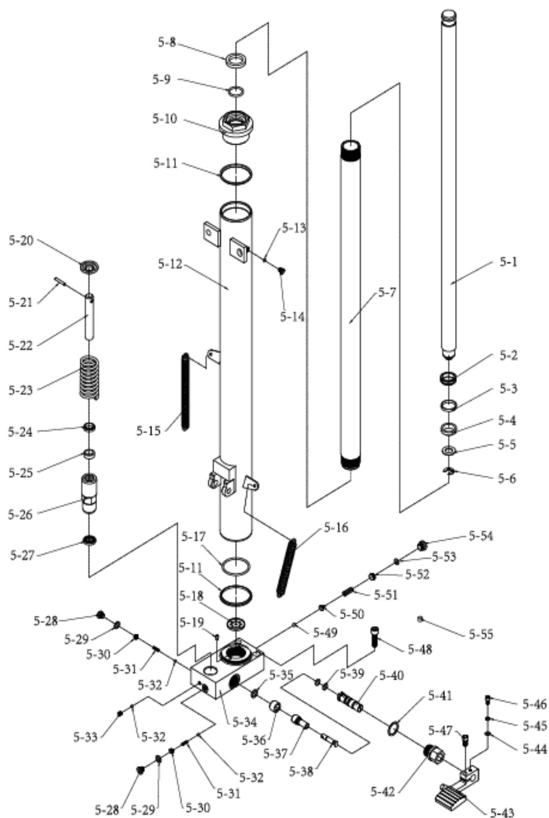
Fig.5 Cylinder assembly
